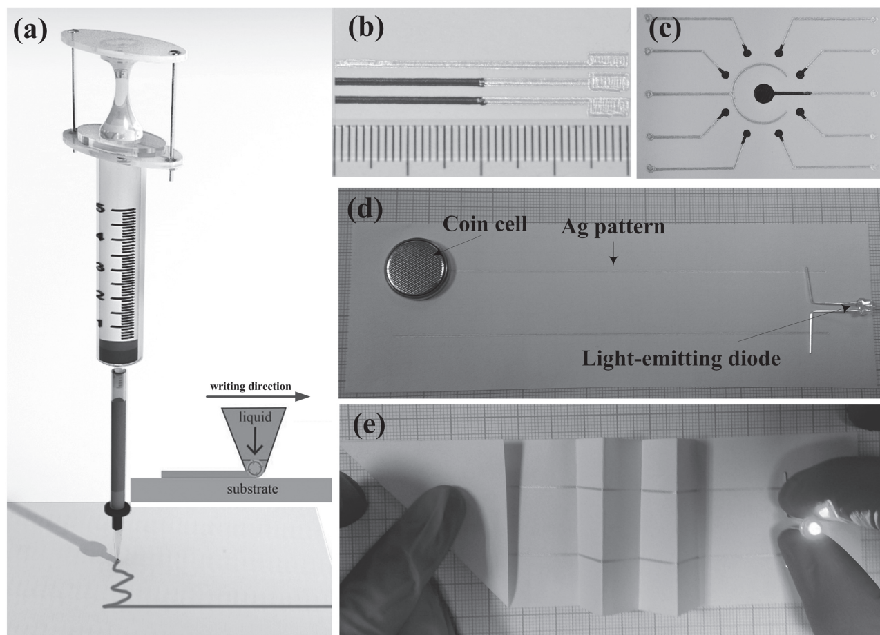
Figure 5. Writing electronics using a ball pen. a) Schematic diagram of direct writing electronics on paper using a pressure-assisted ball pen, the inset showing the working principle of the ball pen writing. b,c) Photographs of fabricated paper based electrochemical devices with b) a three electrode system of a carbon working electrode, silver reference electrode, and carbon counter electrode and c) an eight-electrode array of eight carbon working electrodes, a communal silver reference electrode, and a communal carbon counter electrode. d) The photograph of a closed loop with a coin cell and a LED connected by the written silver traces. e) The LED lights to show that the written silver traces retain conductive even after folding of paper substrate. Reproduced with permission. [52] Copyright 2015, Royal Society of Chemistry. Reproduced with permission. [34] Copyright 2014, Nature Publishing Group.
